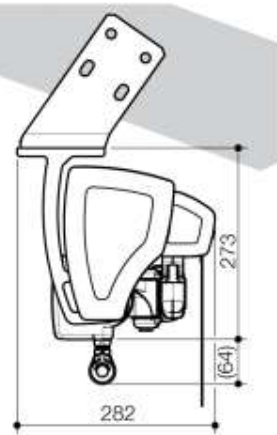
Rafter installation
