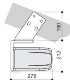
Rafter installation
